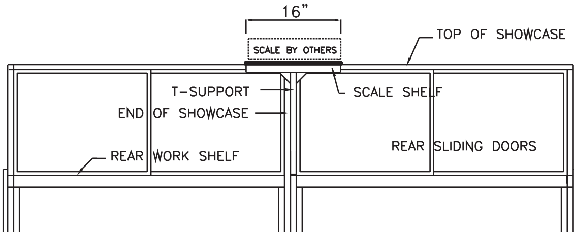
REAR ELEVATION
